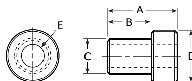
NB CONCENTRIC BUSHING
