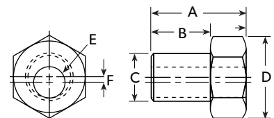
NBX ADJUSTABLE BUSHING
